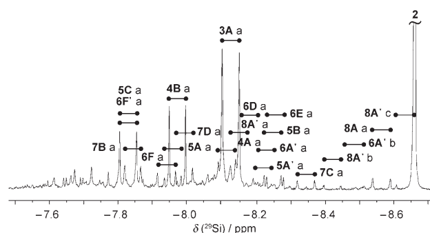
Figure 4. Expanded ^{29}\text{Si} NMR one-dimensional spectrum of the potassium silicate solution from Figure 2 at 272 K, showing the end-group spectral region.
