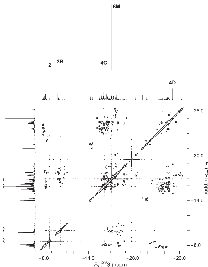
Figure 2. ^{29}\text{Si} NMR one-dimensional and COSY spectra (149 MHz) at 280 K of an aqueous potassium silicate solution containing 1.0 \text{ mol kg}^{-1} \text{SiO}_2 (enriched 99.35 atom% in ^{29}\text{Si} ) and 1.0 \text{ mol kg}^{-1} KOH. The entire spectrum is shown except for the orthosilicic acid resonance at 0 ppm, for which there is no cross-peak. Resonances corresponding to single-site silicate species are labeled in accordance with Figure 1.
