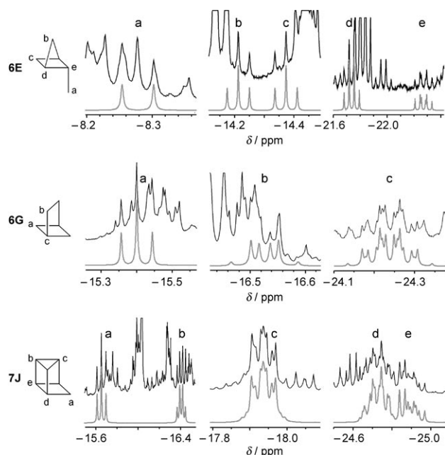
Figure 3. Expanded 1D ^{29}\text{Si} NMR spectrum from Figure 2. The resonances corresponding to species 6E (3-trihydroxysilylbicyclo[3.3.3]pentasilicic acid), 6G (bicyclo[5.3.3]hexasilicic acid), and 7J (tetracyclo[7.5.1.1 3,7 .1 5,11 ]heptasilicic acid) are displayed, along with their computer-modeled simulations (shown in gray).
